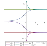
Figure 7.7: Graficul orbite: x' = x - x^3
