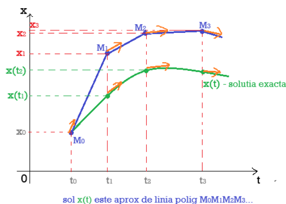
Figure 13.1: Metoda liniilor poligonale
